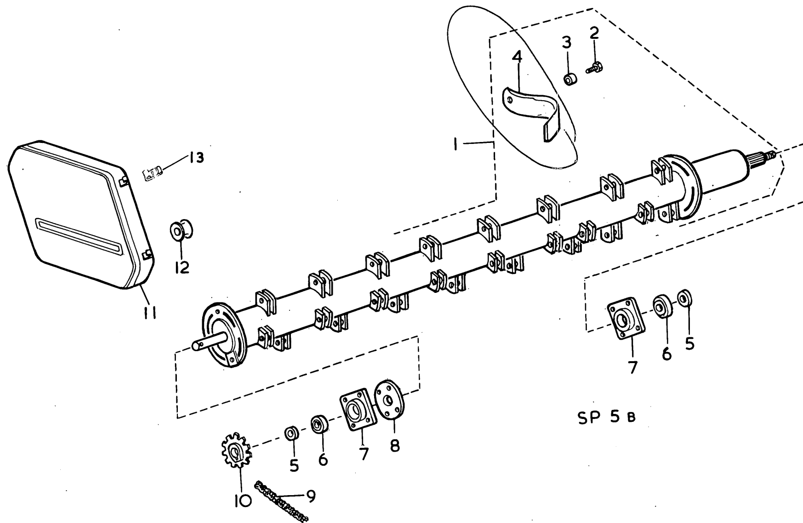
37 DOUBLE - CHOP ROTOR GROUP
